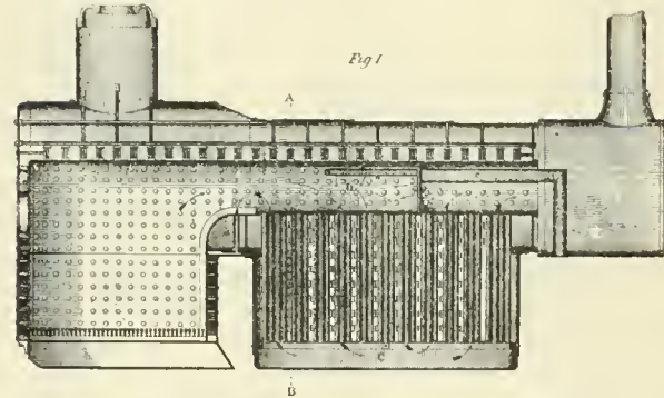
BOARDMAN'S BOILER. FIG. 71.
